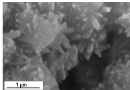
Figure 1. SEM micrograph of \text{Ca(OH)}_2 commercial particles reacted at 333 K, 70% RH and 2000 ppm of \text{SO}_2 for 2 h.
