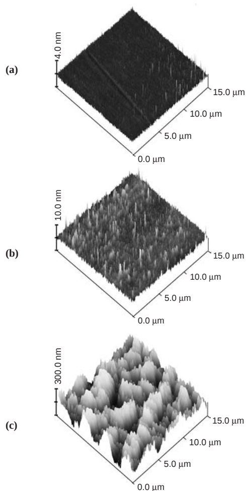
Figure 2. TM-AFM images of freshly cleaved \text{Ca(OH)}_2 (0001) surfaces reacted at 313 K and 5500 ppm of \text{SO}_2 for 30 min. (a) Freshly cleaved surface, Rms: 0.1 nm; (b) 15% RH, Rms: 1.1 nm; (c) 70% RH, Rms: 59.6 nm.
