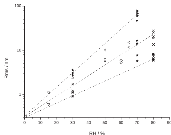
Figure 3. Dependence of the surface roughness of cleaved \text{Ca(OH)}_2 (0001) surfaces on the RH for 30 min of reaction. Each symbol indicates different regions of the same crystal.
