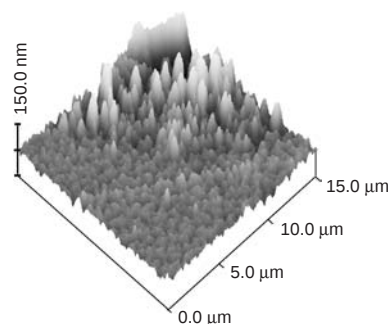
Figure 4. TM-AFM image of a freshly cleaved \text{Ca(OH)}_2 (0001) surface reacted at 313 K, 5500 ppm of \text{SO}_2 and 80% RH for 30 min, where two adjacent regions with surface Rms (5.2 and 26.7 nm) can be distinguished.
